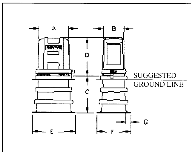
Figure 3. Polymer Secondary Pedestal Dimensions.
